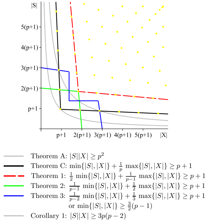
FIGURE 2. Bound comparison.
