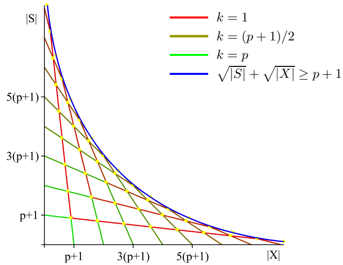
FIGURE 1. Conjecture 1.
