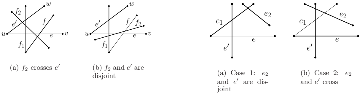
Figure 2: Illustrations for the proof of Lemma 3.4
