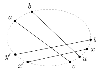
Figure 6: An illustration for the proof of Theorem 4.2
