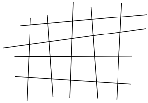
Figure 1: a “natural” grid
