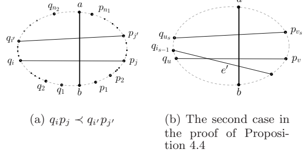
Figure 7: Illustrations for the proof of Theorem 4.3
