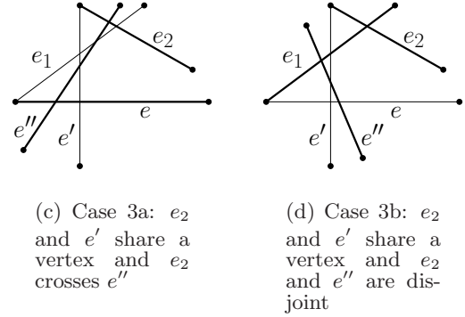
Figure 3: Illustrations for the proof of Lemma 3.6
