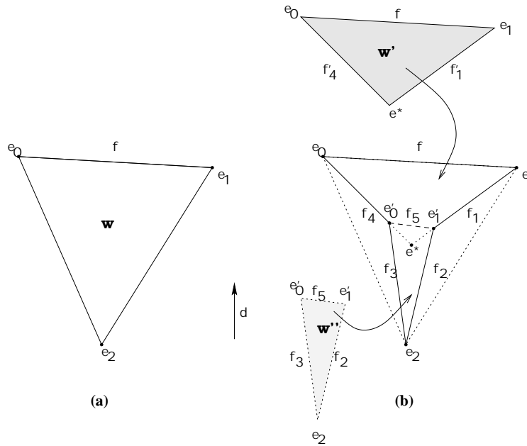
Figure 6: First canonization stage of trihedral wedges. The good direction d is upwards (within the page). (a) A cross section of w by a plane parallel to d . (b) The same cross section after the folding.
