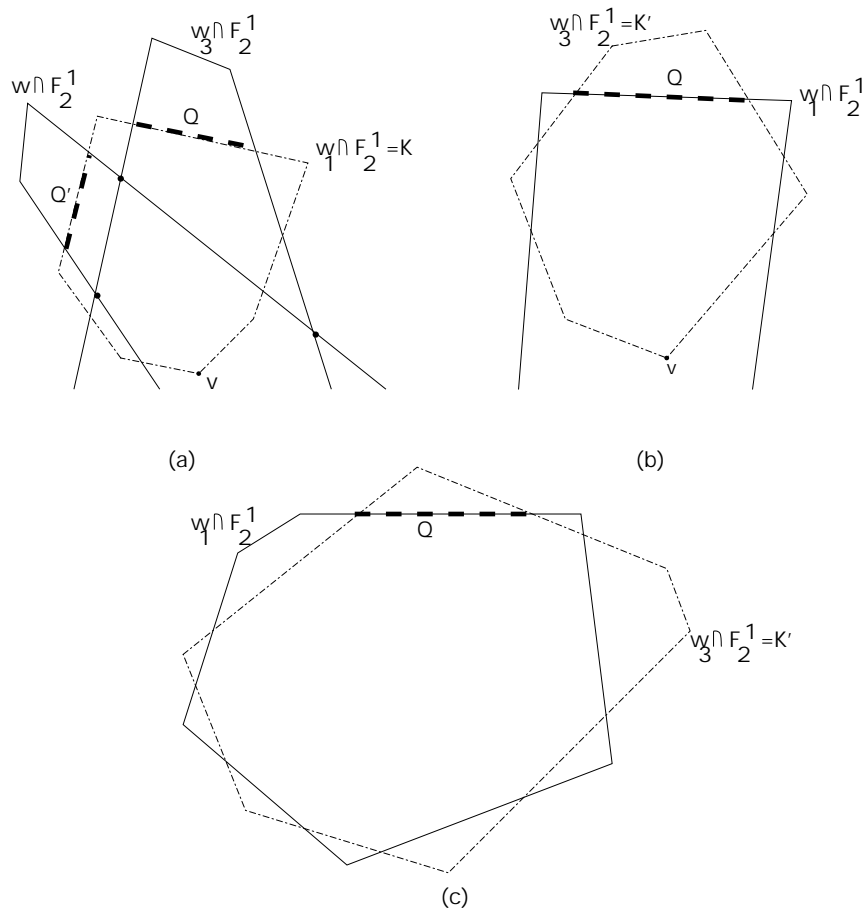
Figure 8: The cases where \varphi is not a quadrilateral: (a) \varphi has a vertex lying on an edge of w_1 ; (b) \varphi has a vertex lying on an edge of w_3 ; (c) \partial\varphi alternates between edges lying on \partial w_1 and edges lying on \partial w_3 .
