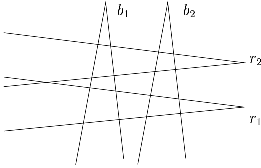
Figure 4: r_2 is initial for b_2 , whereas r_1 is not. Each red wedge is semi-free within every blue wedge, and vice versa.
