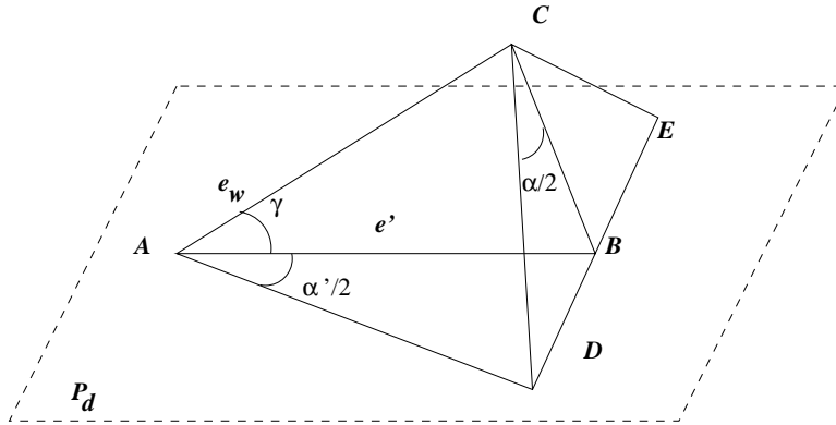
Figure 1: The setup in the proof of Lemma 2.2.
