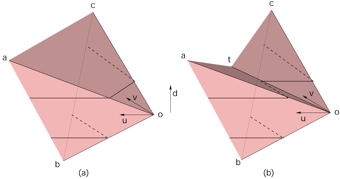
Figure 7: The cross sections of a trihedral wedge w by planes in a good direction: (a) for the original w ; (b) after folding inwards a face of w .
