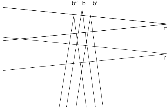
Figure 5: Since r is semi-free within b , the two blue neighbors b', b'' cannot overlap along \partial r .
