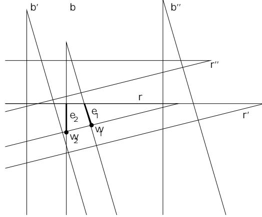
Figure 2: The cross section of a two-colored special cube, at the time when the top edges of r, r' overlap. The bottom vertices w_1, w_2 lie inside r' only and on the boundaries of r and b .
