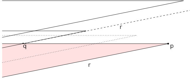
Figure 3: No red 2-wedge above r can have a point below \rho , the dashed ray emanating from q to the right. Thus, the apex of any long blue wedge with respect to r lies above \rho .
